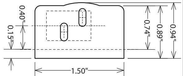
Solenoid Bracket
